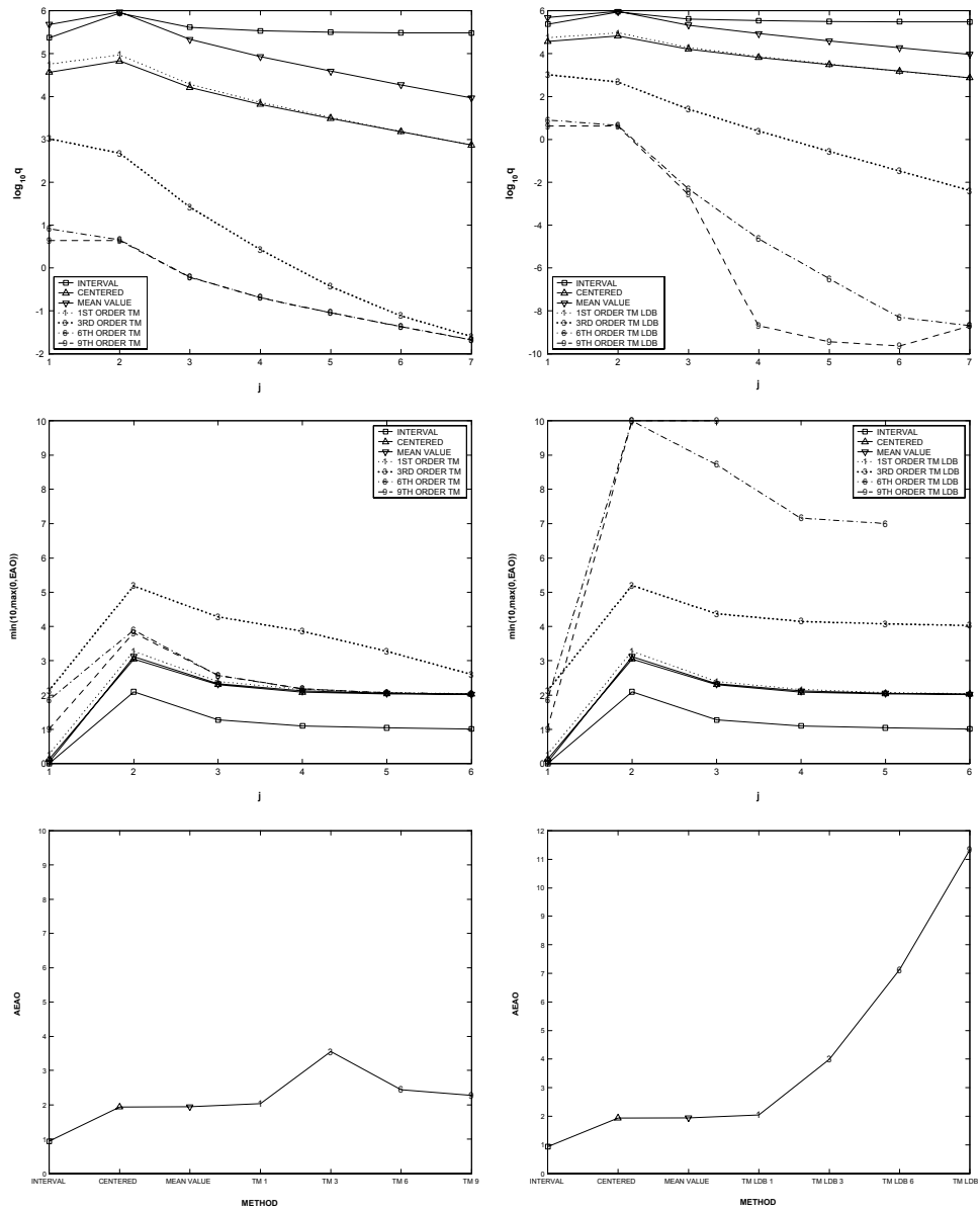
Figure 5: q , EAO and ABAO for the Gritton function f_3(x) around the expansion point x_0 = 2 , without LDB (left), with LDB (right).
