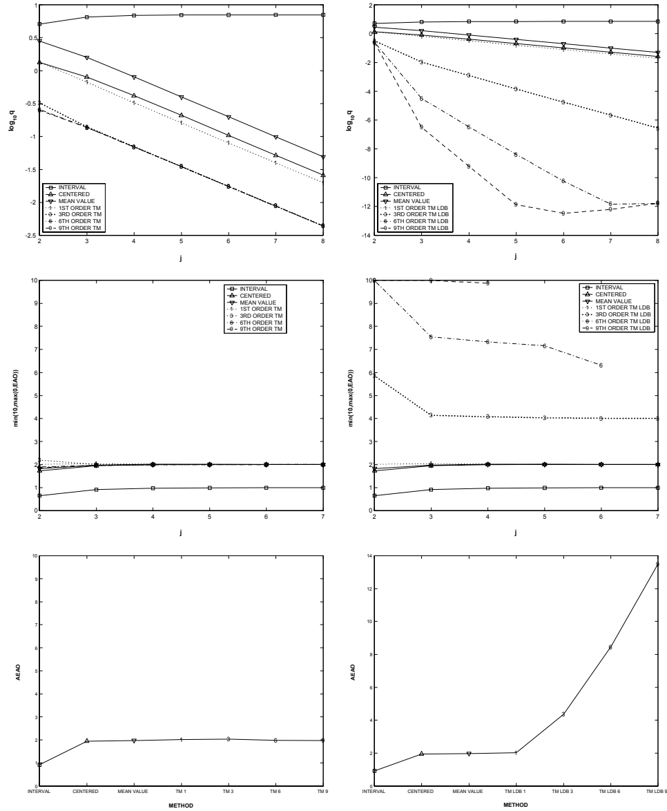
Figure 3: Relative overestimation q , EAO and AEA0 for the function f_1(x, y, z) in the domain (2, 1, 1) + [-2^{-j}, 2^{-j}] , without LDB (left), with LDB (right).
