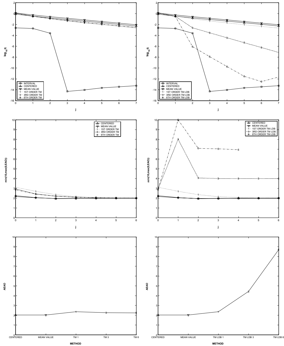
Figure 9: q , EAO and AEAO for the 10D function f_5(\vec{x}) around the expansion point \vec{x}_0 = 1.75^{10} , without LDB (left), with LDB (right).
