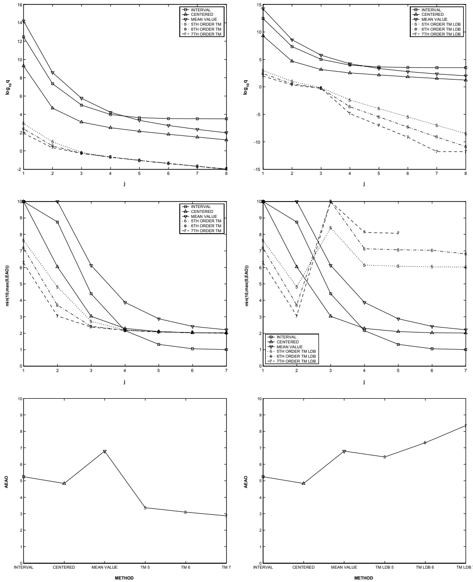
Figure 7: q , EAO and AEO for the 6D normal form deviation function f_4(\vec{x}) in the domain 0.1 \cdot (1 + [-2^{-j}, 2^{-j}])^6 , without LDB (left), with LDB (right).
