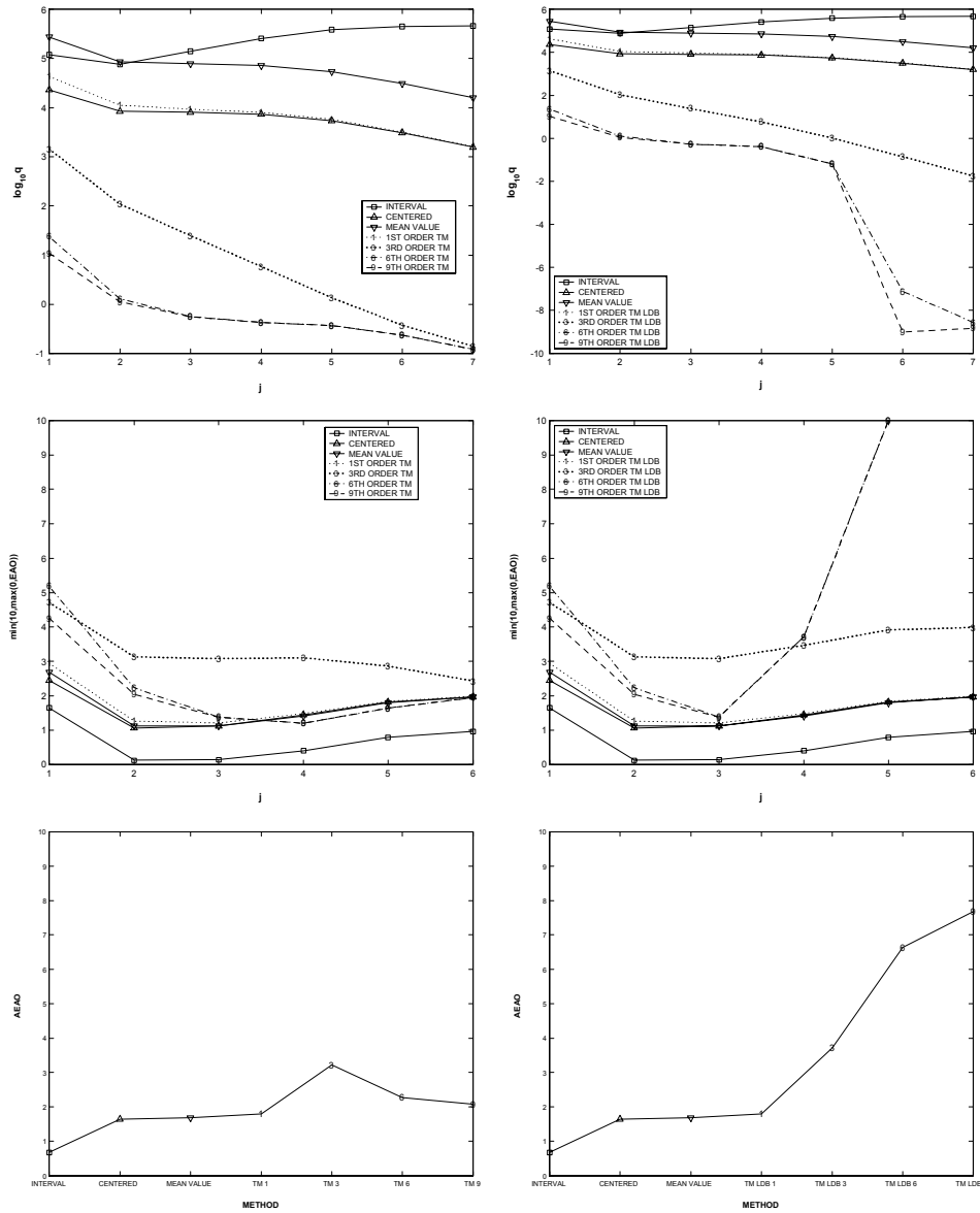
Figure 6: q , EAO and AEAQ for the Gritton function f_3(x) around the expansion point x_0 = 1.4 where the cancellation problem is very significant, without LDB (left), with LDB (right).
