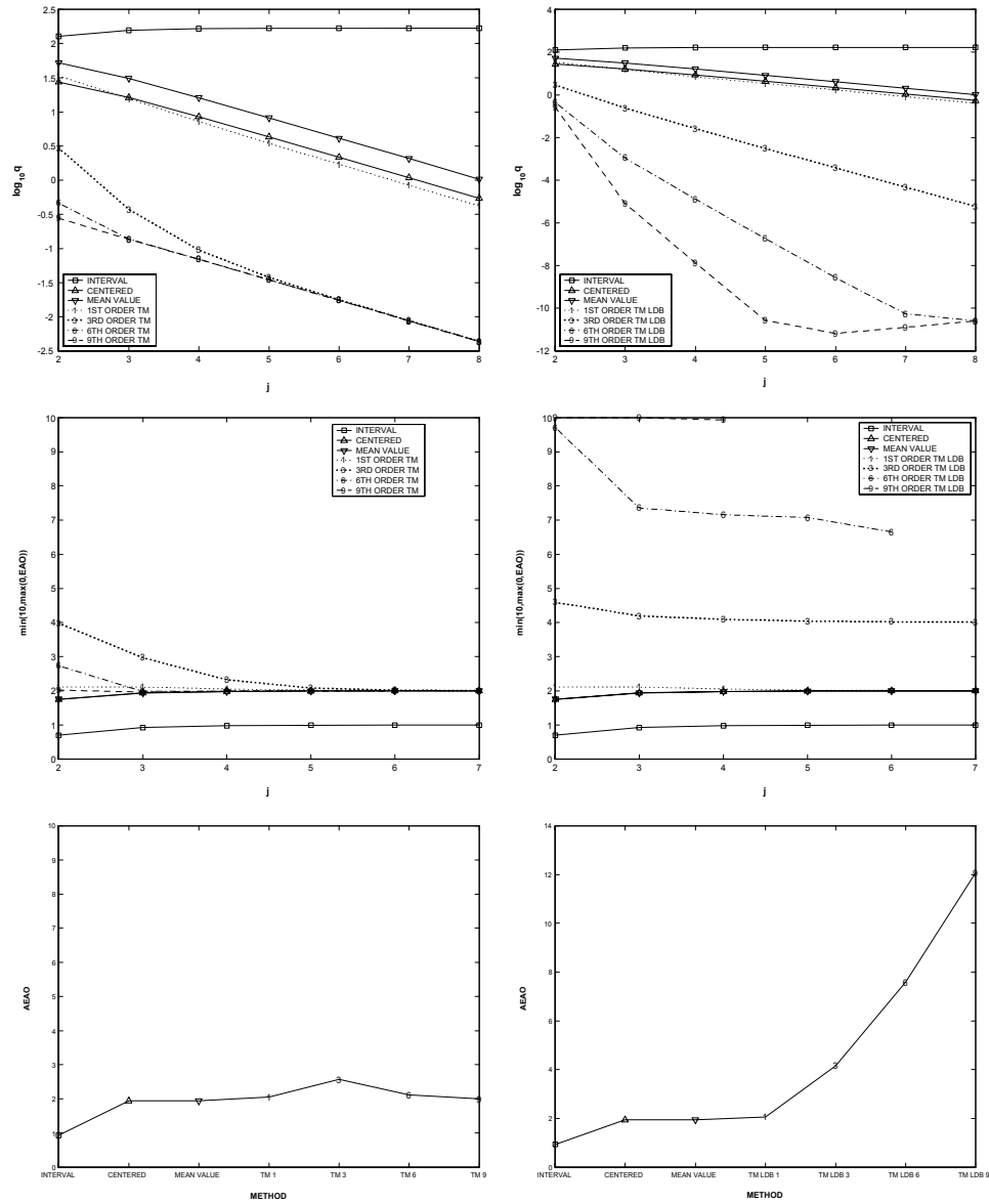
Figure 4: q , EAO and ABAO for the repeated function f_2(x, y, z) in the domain (2, 1, 1) + [-2^{-j}, 2^{-j}] , without LDB (left), with LDB (right).
